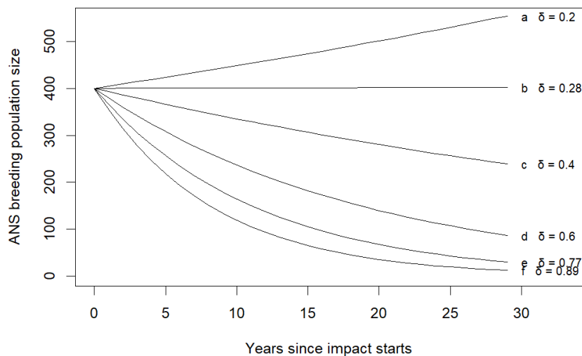
Figure C: Realised population dynamics of a hypothetical ANS with 400 breeding pairs in year 1 at different levels of net natal dispersal \delta (using first year and adult survival rates \phi of 0.79 and 0.854, respectively and a productivity of F=0.819 ). a–f show a selection of different dispersal rates (b is the maximum sustainable dispersal at F=0.819 ; e,f are the dispersal rates assumed in Hornsea 3 approach).
